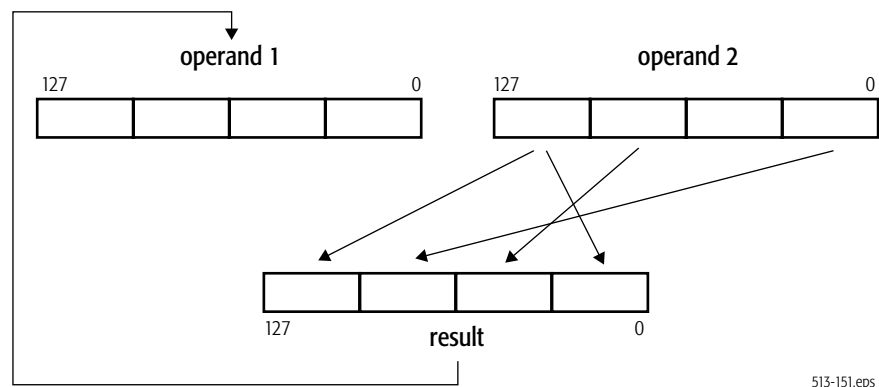
Figure 4-5. Shuffle Operation
