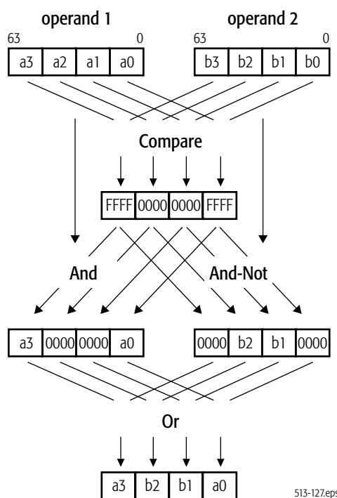
Figure 5-5. Branch-Removal Sequence
