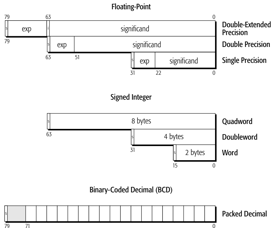
Figure 6-7. x87 Data Types
