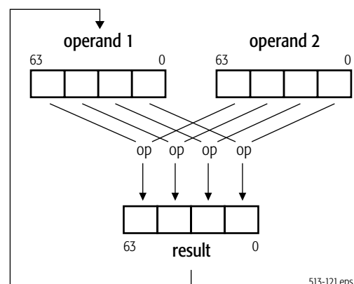
Figure 5-1. Parallel Integer Operations on Elements of Vectors
